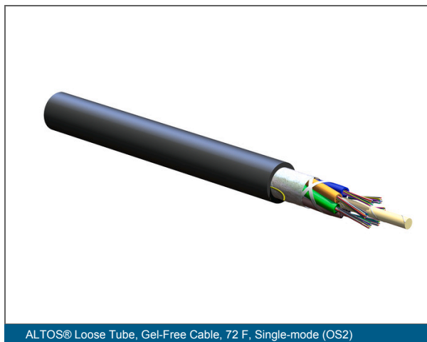
ALTOS® Loose Tube, Gel-Free Cable, 72 F, Single-mode (OS2)
