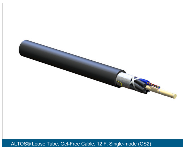
ALTOS® Loose Tube, Gel-Free Cable, 12 F, Single-mode (OS2)
