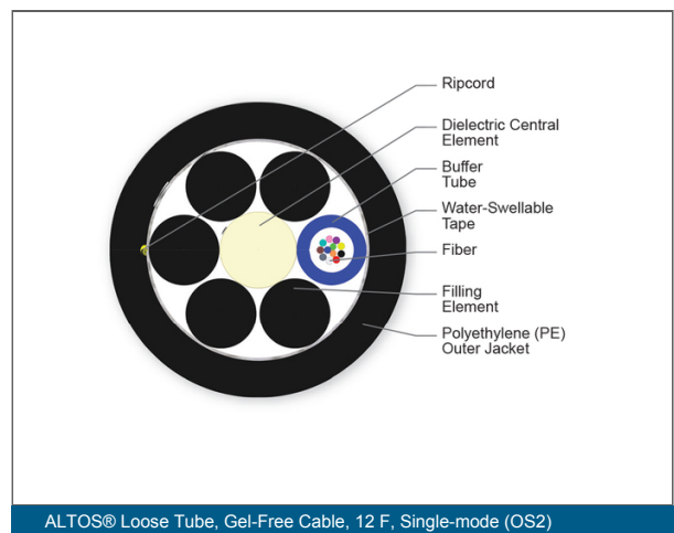
ALTOS® Loose Tube, Gel-Free Cable, 12 F, Single-mode (OS2)
